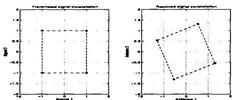
Figure 1: Transmitted and received signal constellations
