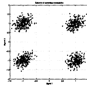
Figure 4: Estimate of transmitted constellation
