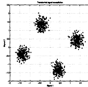
Figure 3: Transformed signal constellation
