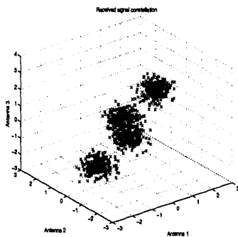
Figure 2: Received signal constellation
