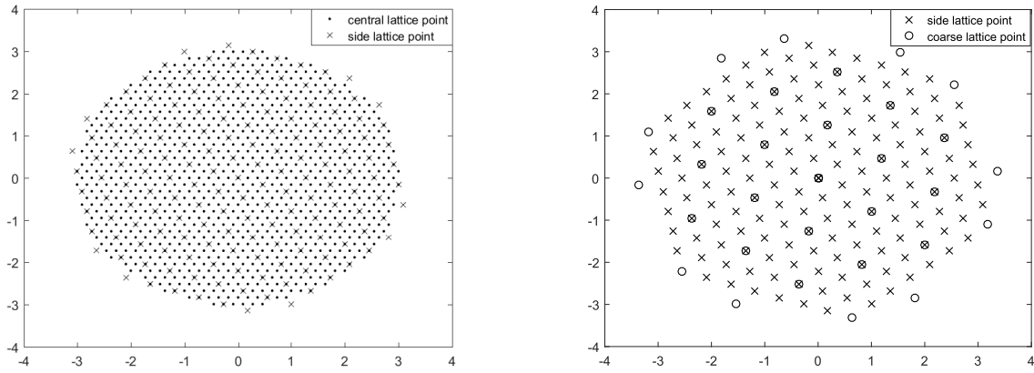
Fig. 4. The sets \mathcal{B}_c , \mathcal{B}_1 , \mathcal{B}_2 and \mathcal{B} for Example 2.
