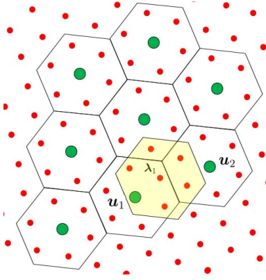
Fig. 2. Partitioning using Voronoi regions of the coarse lattice. The small red-filled circles are points of \Lambda_s , while big green-filled circles represent points of the coarse lattice \Lambda \subset \Lambda_s . The hexagons centered at the coarse lattice points are the Voronoi regions of the coarse lattice. The set \lambda_1 + \mathcal{W} (highlighted) contains \lambda_1 and the six side lattice points closest to \lambda_1 and it intersects three Voronoi regions of the coarse lattice.
