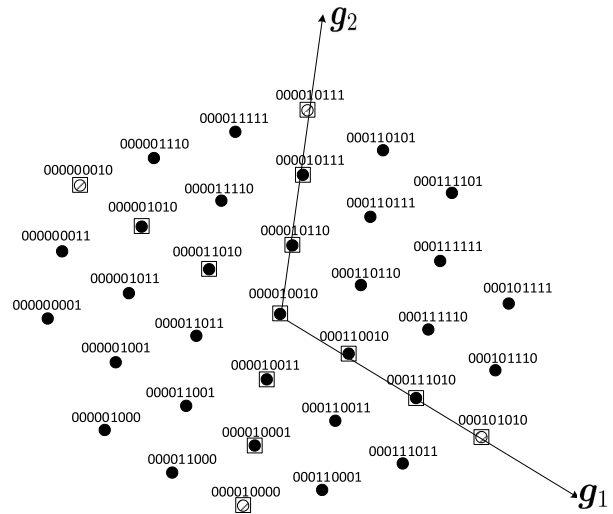
Fig. 5. Mapping \psi_{GM} for Example 2.
