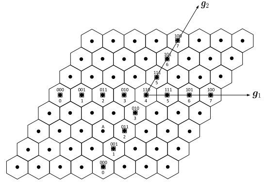
Fig. 3. Illustration of the GMD method.
