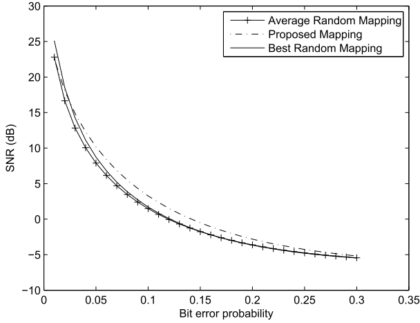
Fig. 7. Performance of the proposed mapping when both channels are noisy.
