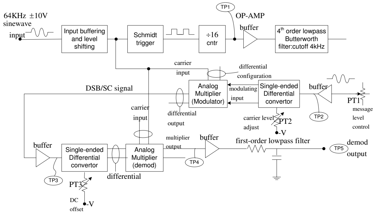
Figure 1 Block diagram of AM modulator-demodulator circuit
