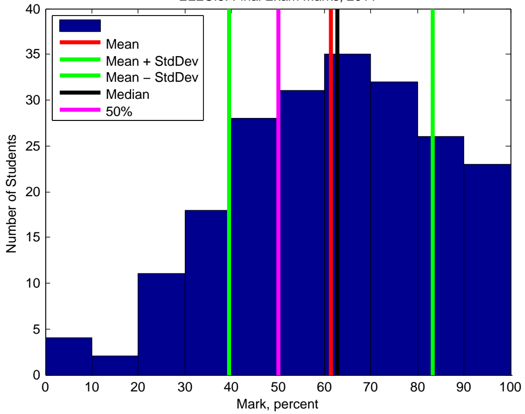
EE2CI5: Final Exam Marks, 2011
