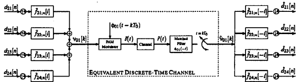
Figure 2: An equivalent model for Fig. 1.
