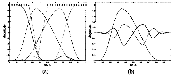
Figure 3: Frequency response of: (a) the equivalent filters for the WPDM scheme and the equivalent notch channel at a particular instant (dotted, with asterisks); (b) the equivalent filters for the (2, 2) terminal for the WPDM scheme (dashed) and the (1:0) strategy (solid and dash-dot); for the schemes in Ex. 1.
