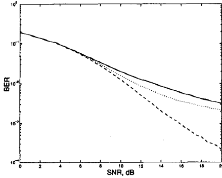
Figure 4: Simulated average BER against Signal-to-Noise Ratio (SNR) for the schemes in Ex. 1. Legend: WPDM and slow BH-WPDM (indistinguishable): solid; (1:0) strategy: dashed; (3:1) strategy: dotted.
