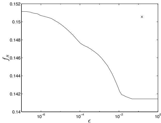
Fig. 7. Minimal stop-band edge f_s against ISI bound \epsilon for the IS95 mask. The ‘ \times ’ denotes the position of the IS95 filter.
