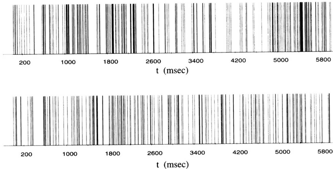
Fig. 15.2 SPIKE TRAINS AND THE RANDOM POISSON PROCESS Spike train from an extracellularly recorded cell in the parietal cortex of a behaving monkey (upper trace; data kindly provided by J. Fuster) and from a synthetic Poisson process with a refractory period of 1 msec (lower trace). The mean firing rate of both processes is 30 Hz. Notice the relatively rare occurrences of large gaps between spikes. In a Poisson process, the probability of occurrence of gaps of duration T decreases as e^{-T\mu} .
