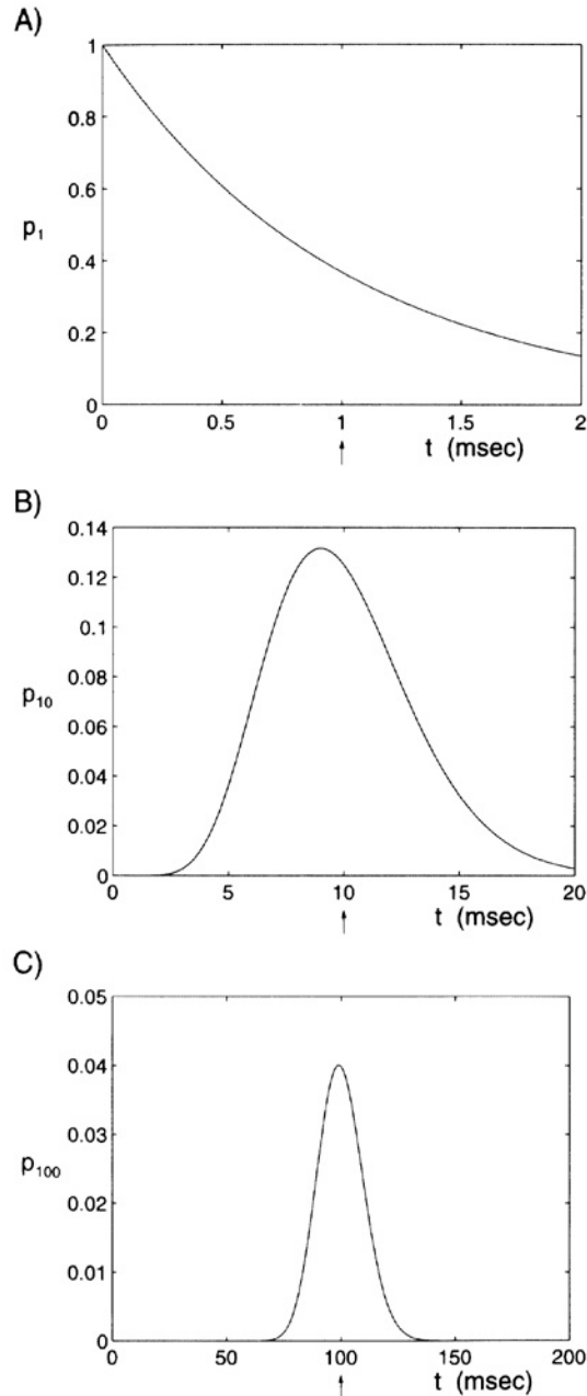
Fig. 15.4 INTERSPIKE INTERVAL DISTRIBUTION
