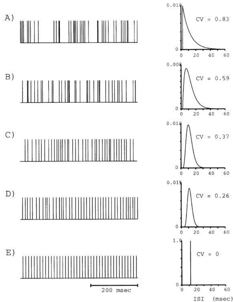
Fig. 15.5 SPIKE TRAIN INTERSPIKE VARIABILITY Sample spike trains and interspike interval histograms for a perfect integrator model with an absolute refractory period t_{\text{ref}} of 2 msec for Poisson distributed synaptic input. The mean interspike interval is in all cases identical to 12 msec. (A) Each synaptic input gives rise to a spike. The ISI is a shifted exponential; the deviation of the associated C_V from unity reflects the regularizing effect of the refractory period. (B)–(D) n_{\text{th}} is increased to 2, 5, and 10, respectively. To retain the same average firing frequency, the input firing frequency was also increased by the same amount. The ISI can be described by a gamma density (Eq. 15.12). (E) Response to a sustained current injection.
