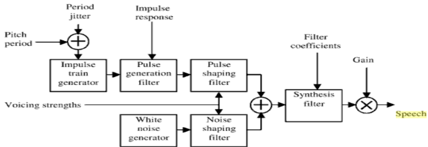
Figure 17.1 The MELP model of speech production.
