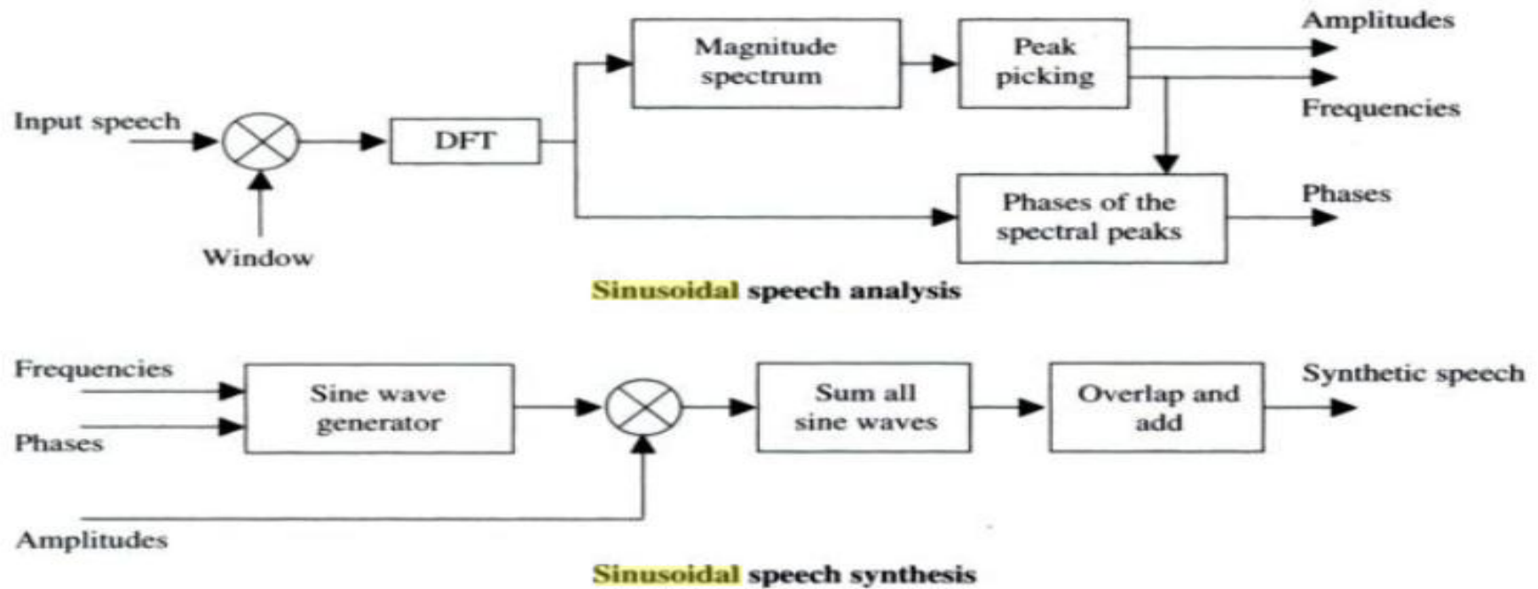
Figure 8.1 General sinusoidal analysis and synthesis
