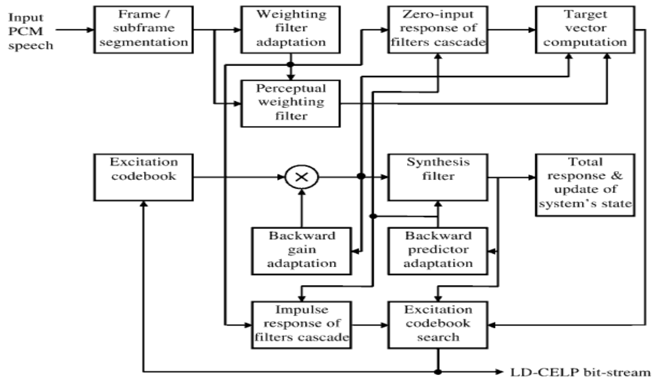
Figure 14.9 Block diagram of the G.728 encoder.
